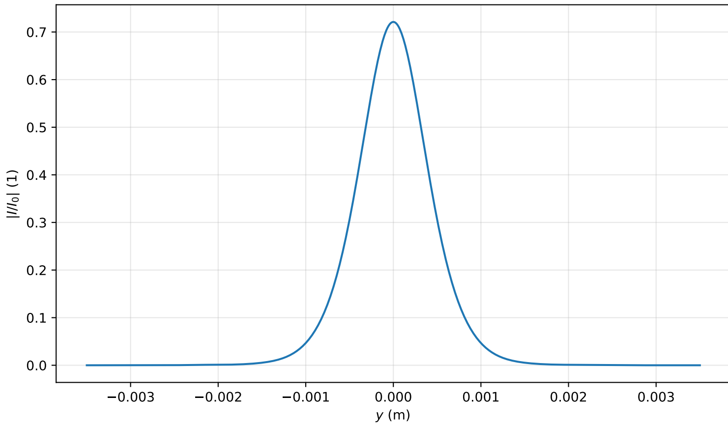
Intensity profile I(x=0, y, z=3.503)/I_0 , P_{in}=0.7P_{cr} , artificial time
